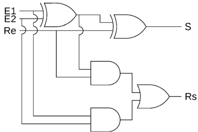
Figure 3. Circuit logique
